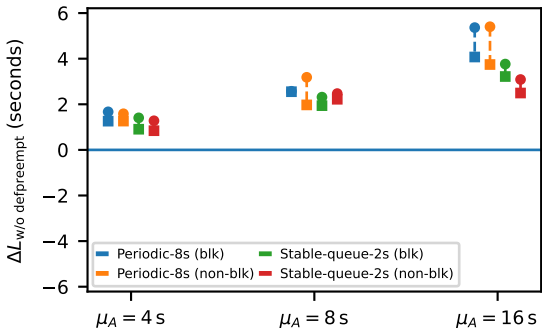
\Delta L_{w/o \text{ defpreempt}} vs \mu_A (kmax=4)
