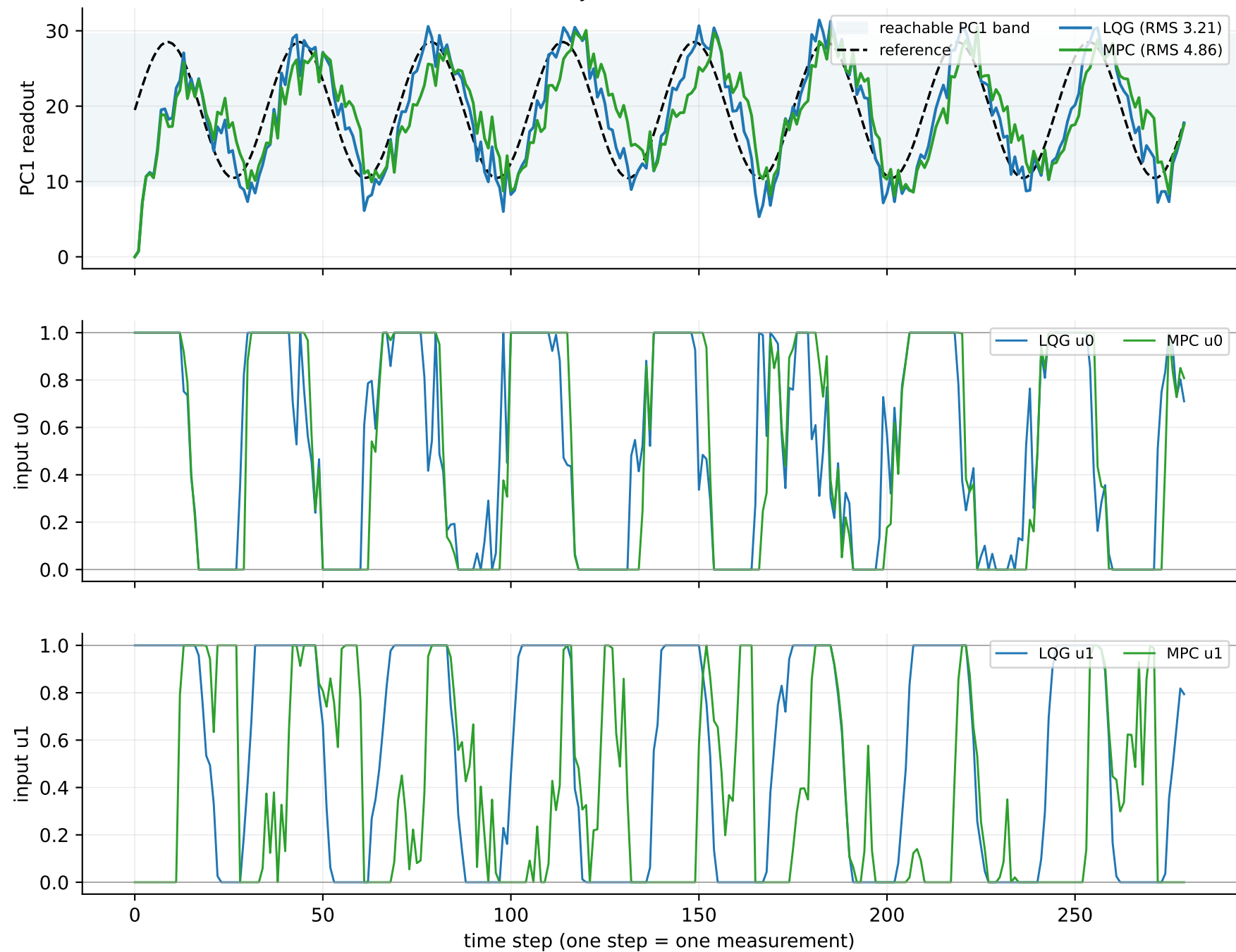
LQG vs MPC - fast boundary reference (PERIOD=35, H=30, rho=1.0)
