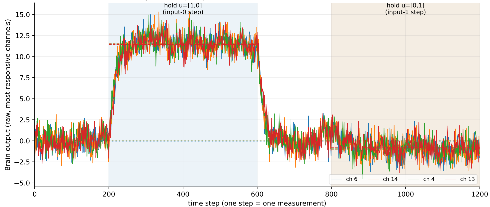
Steady-state step response on the real Brain — Week-4 model validation
