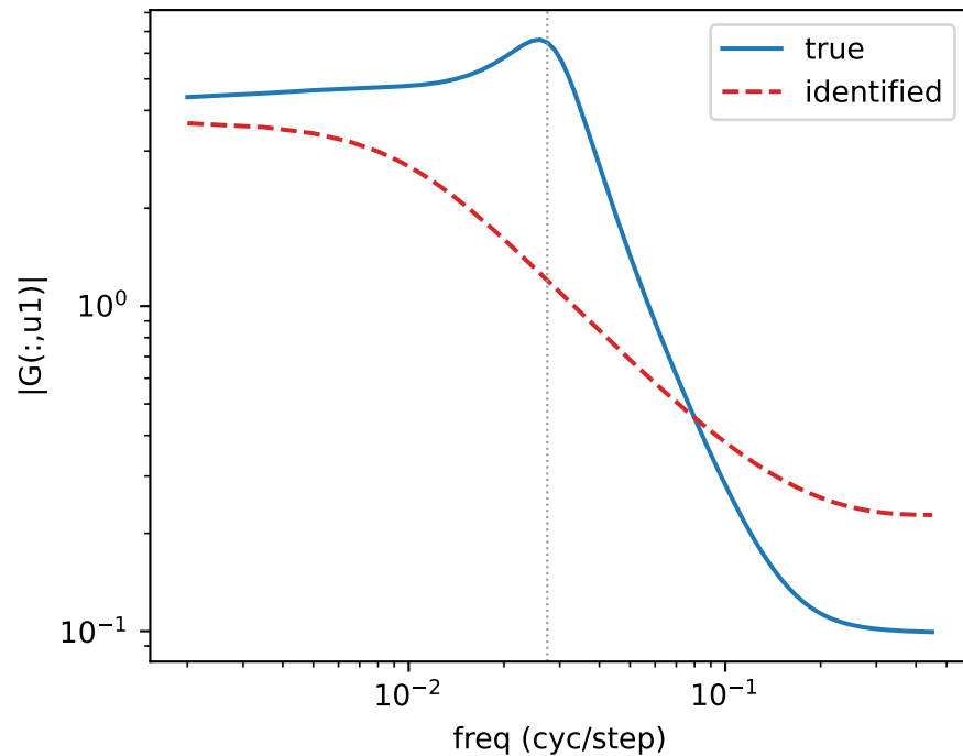
Transfer-function magnitude (resonance marked)
