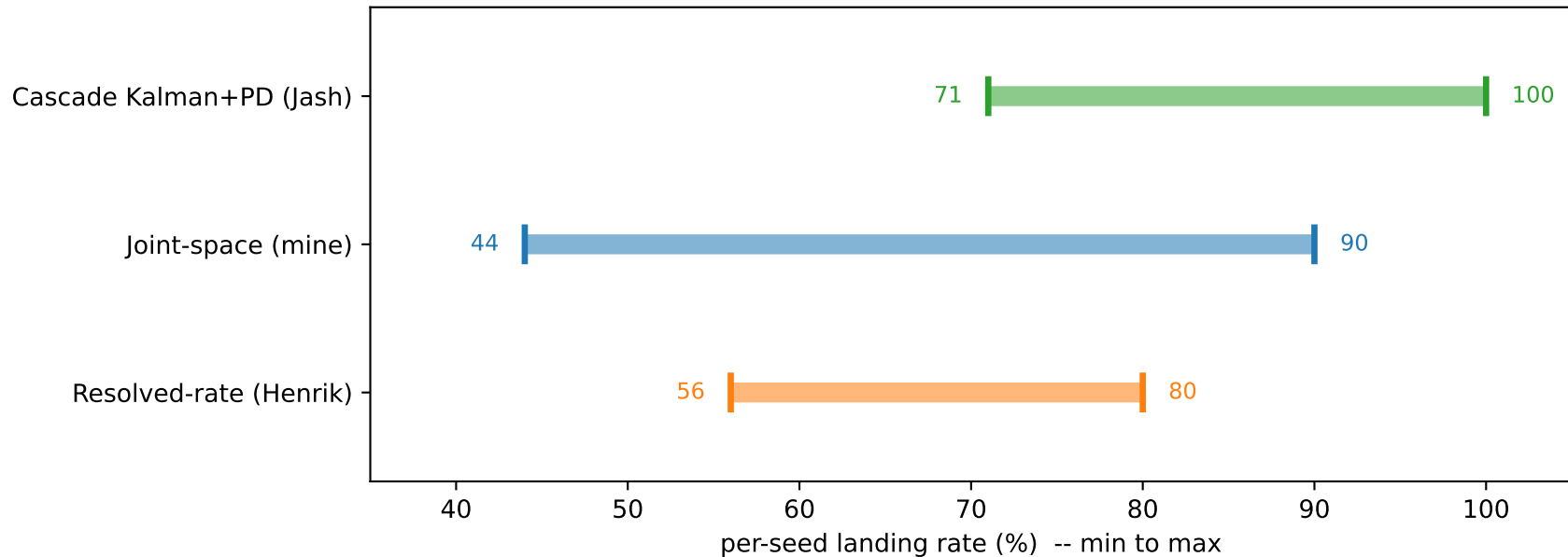
Per-seed landing spread (range across seeds)
