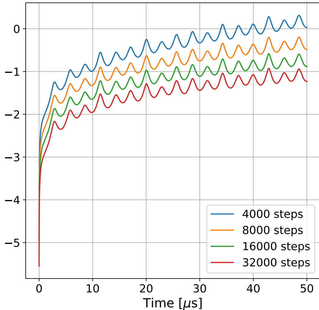
Forward Euler
