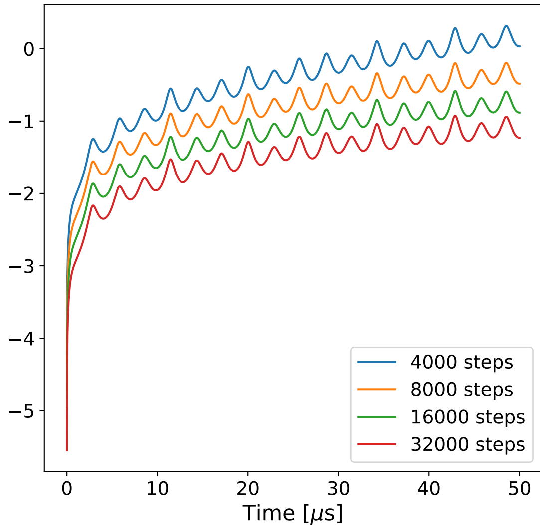
Forward Euler
