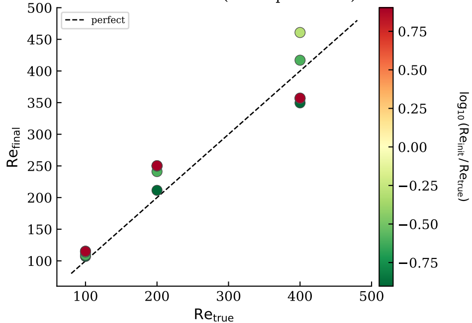
Inferred vs true Re (obs: OpenFOAM)
