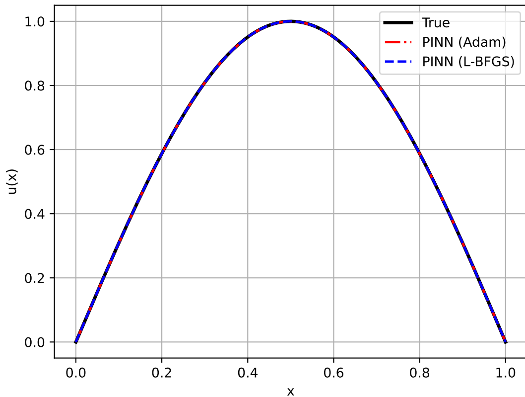
1D Poisson — solution
