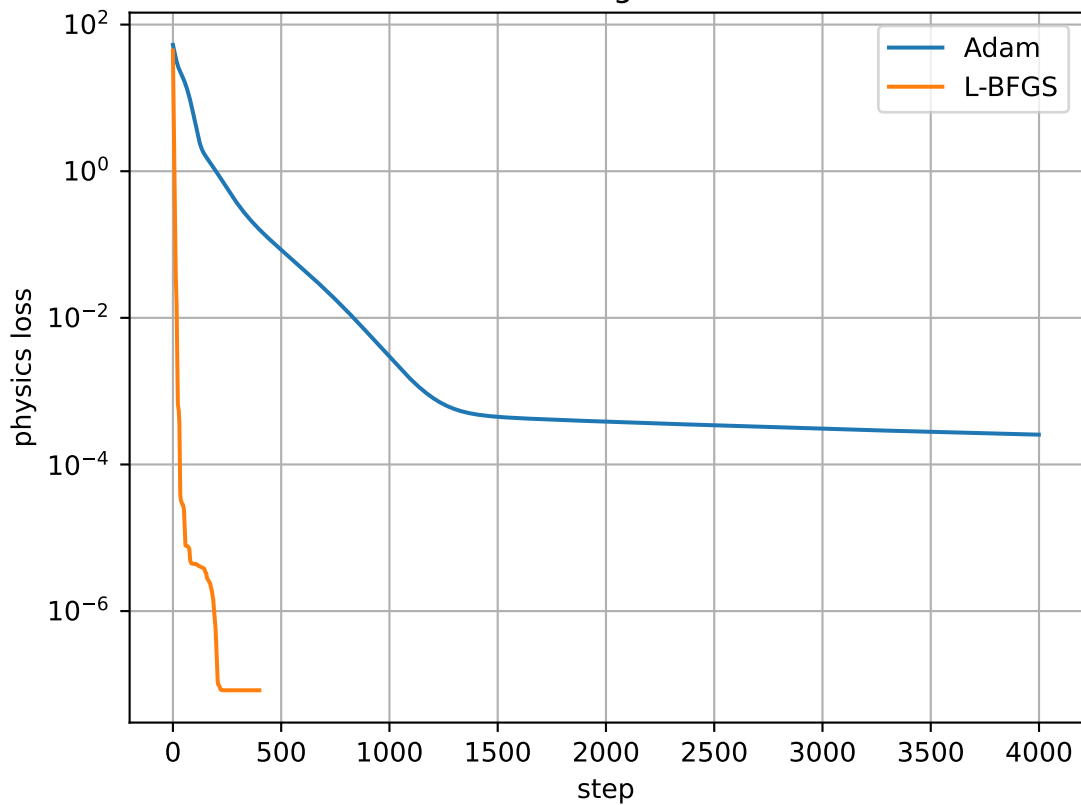
Training loss
