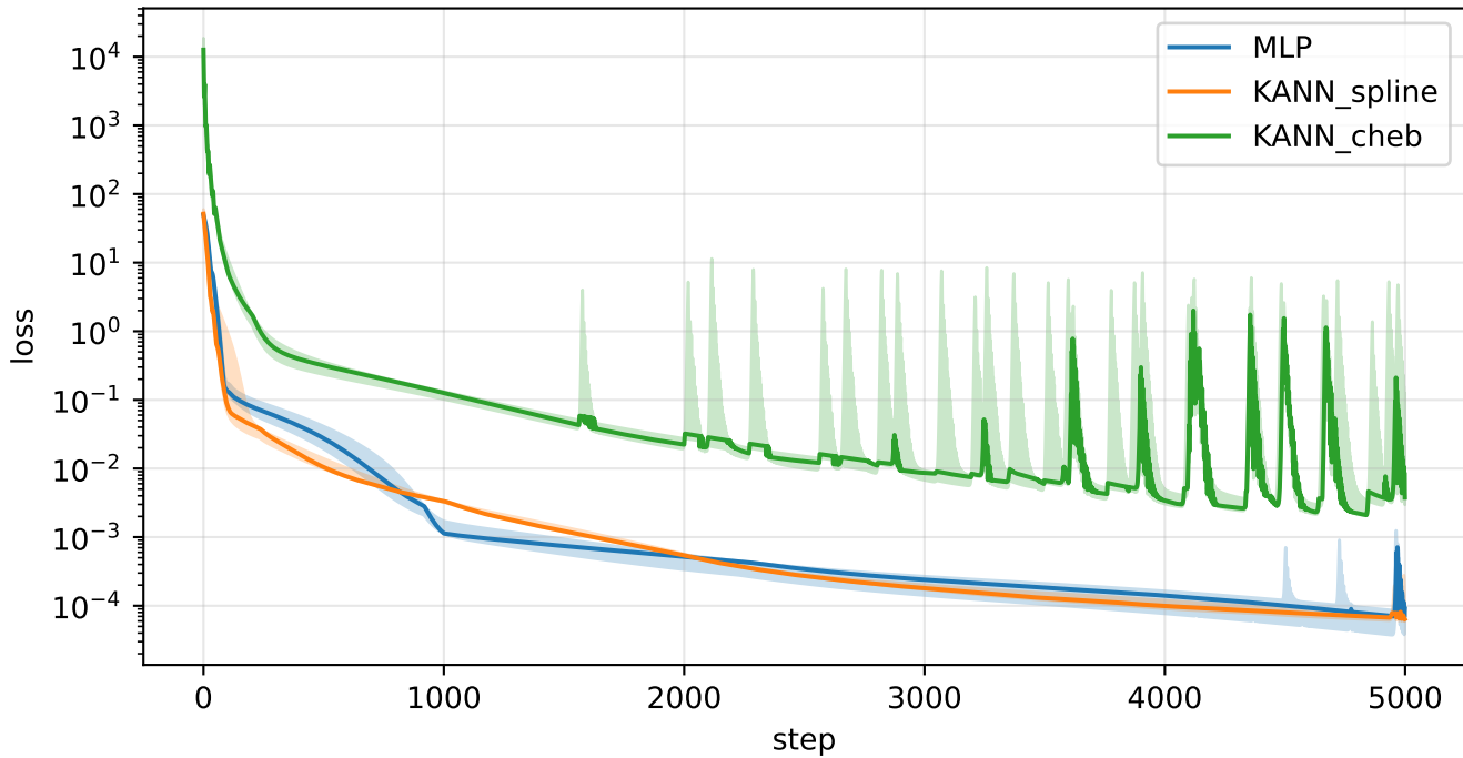
1D Poisson - loss (median over 3 seeds)
