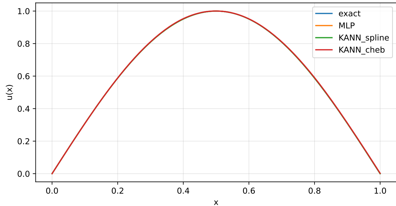
1D Poisson
