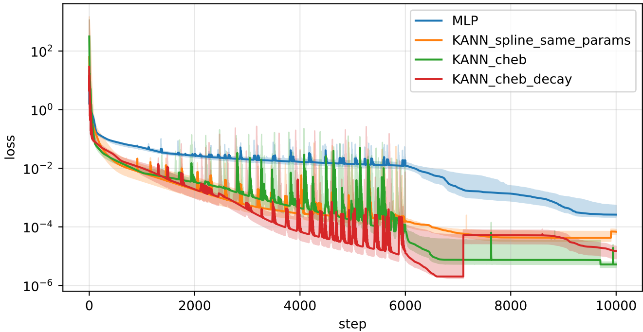
1D Oscillator - loss (median over seeds)
