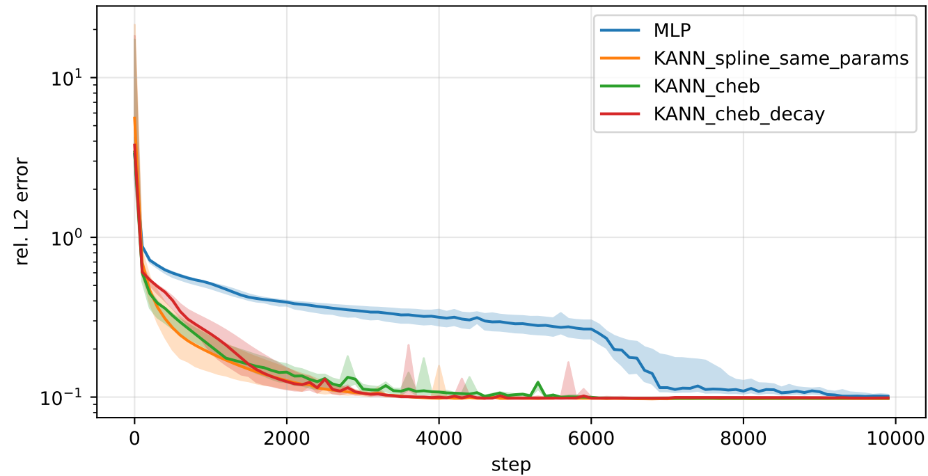
1D Oscillator - relative L2 error (median over seeds)
