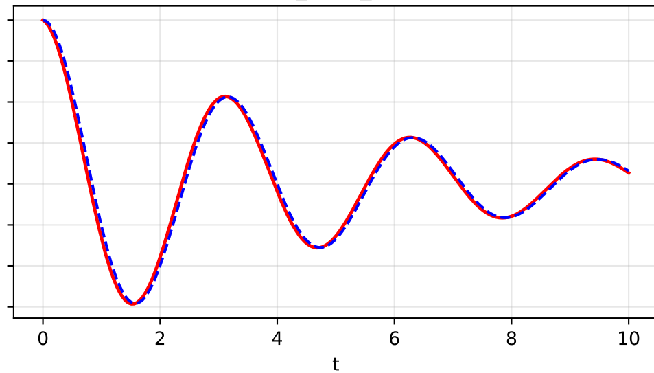
KANN_cheb_decay
