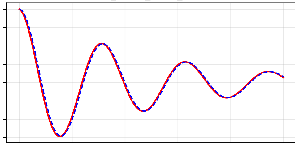
KANN_spline_same_params
