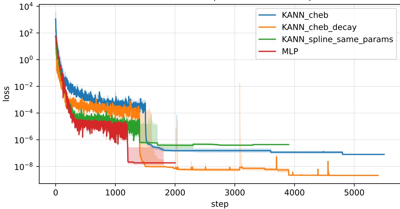
1D Poisson - loss (median over seeds)
