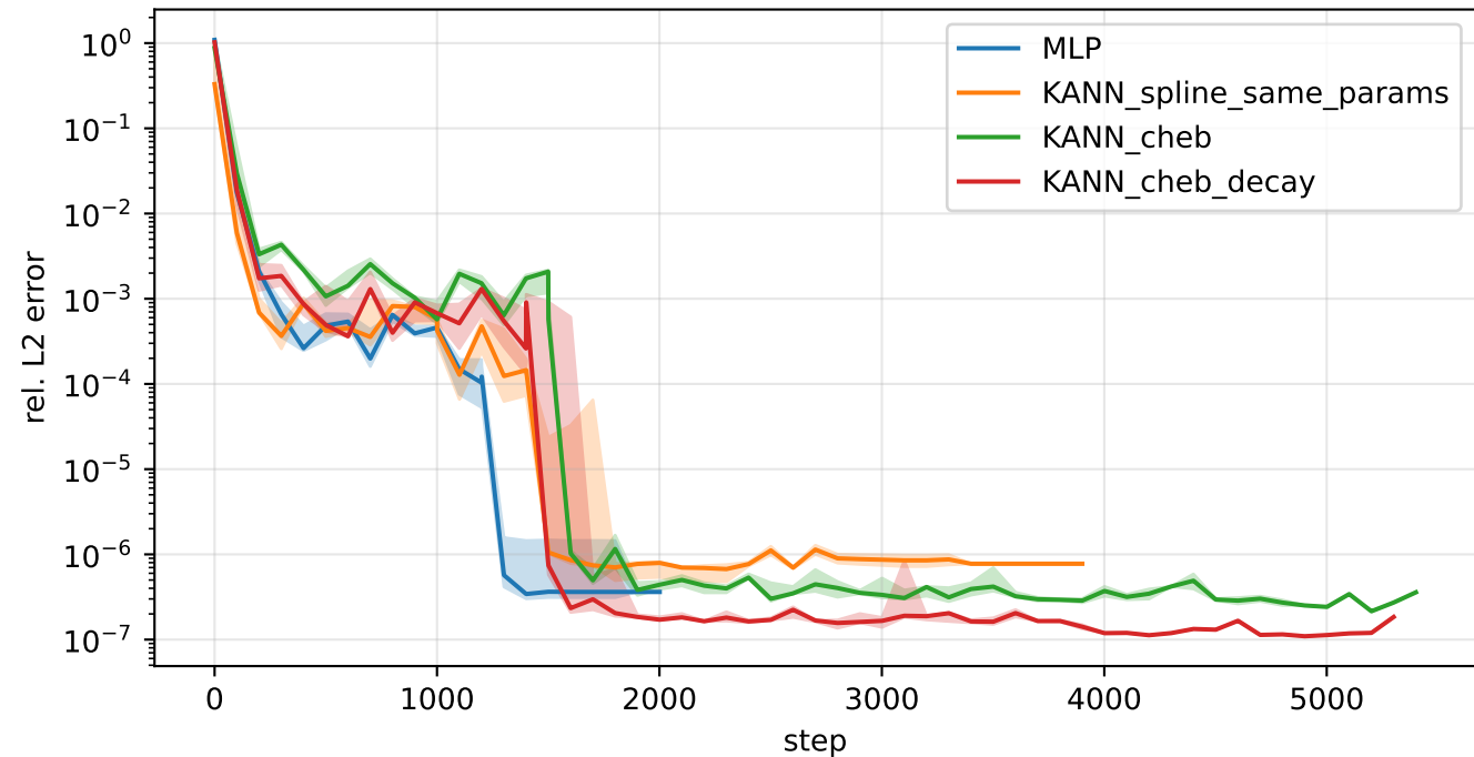
1D Poisson - relative L2 error (median over 3 seeds)
