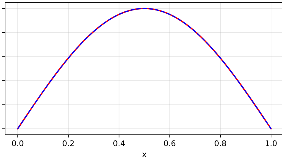
KANN_cheb_decay
