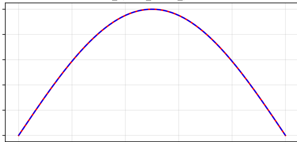
KANN_spline_same_params
