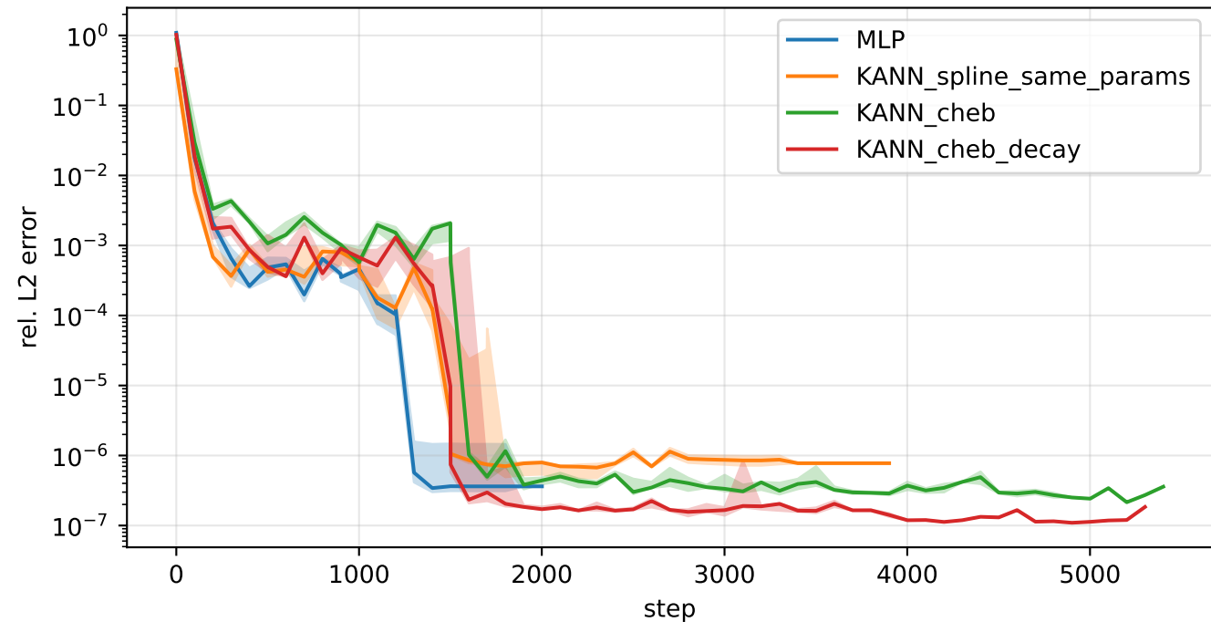
1D Poisson - relative L2 error (median over seeds)
