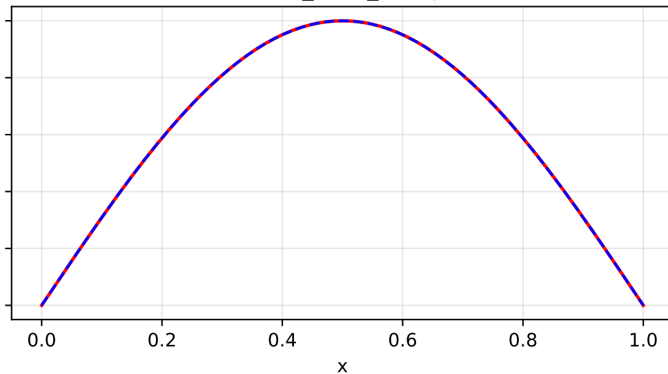
KANN_cheb_decay
