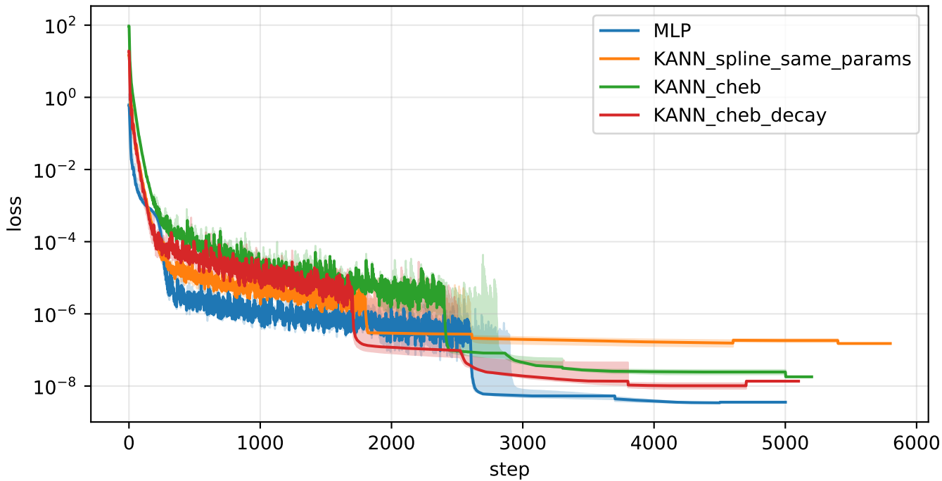
1D Wave Equation - loss (median over 3 seeds)
