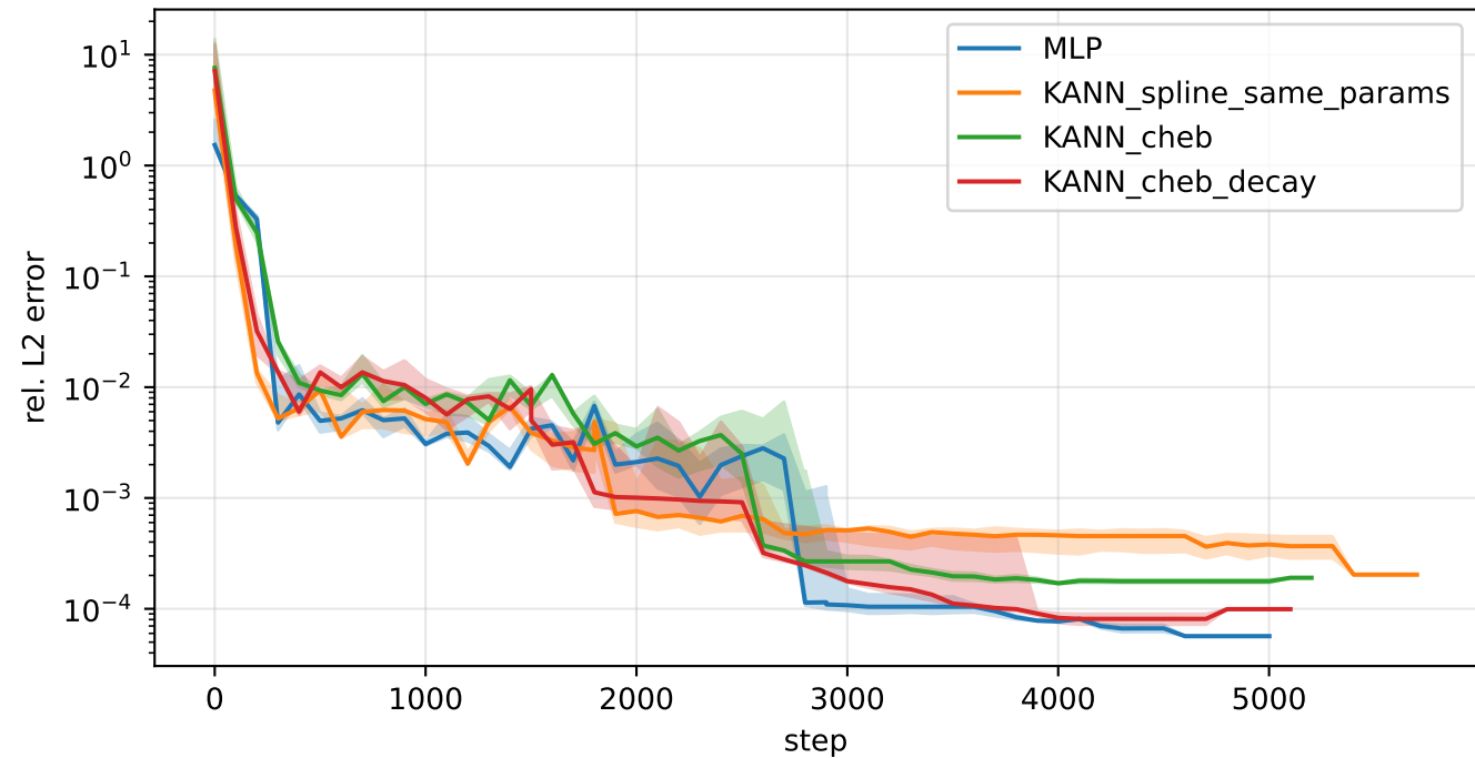
1D Wave Equation - relative L2 error (median over 3 seeds)
