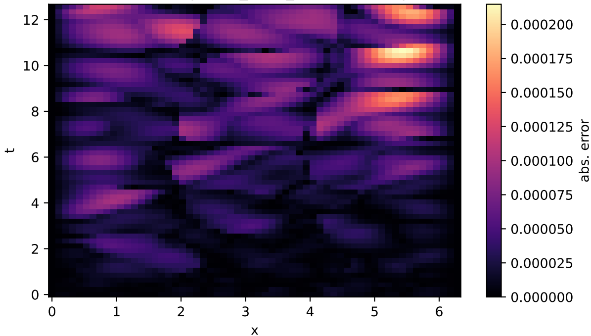
1D Wave - |KANN_cheb_decay - exact|
