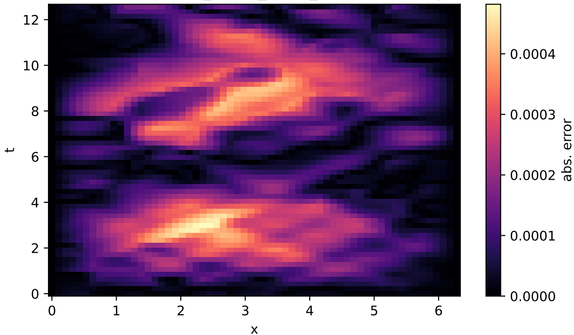
1D Wave - |KANN_spline_same_params - exact|
