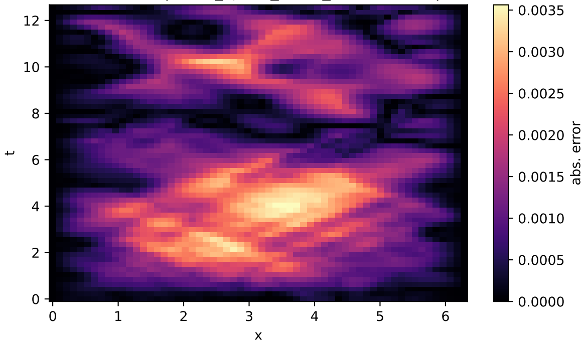
1D Wave - |KANN_spline_same_width - exact|
