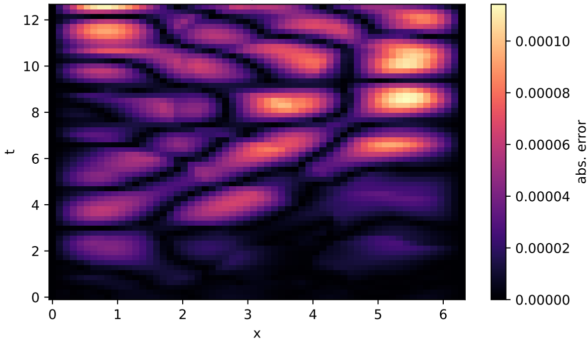
1D Wave - |MLP - exact|
