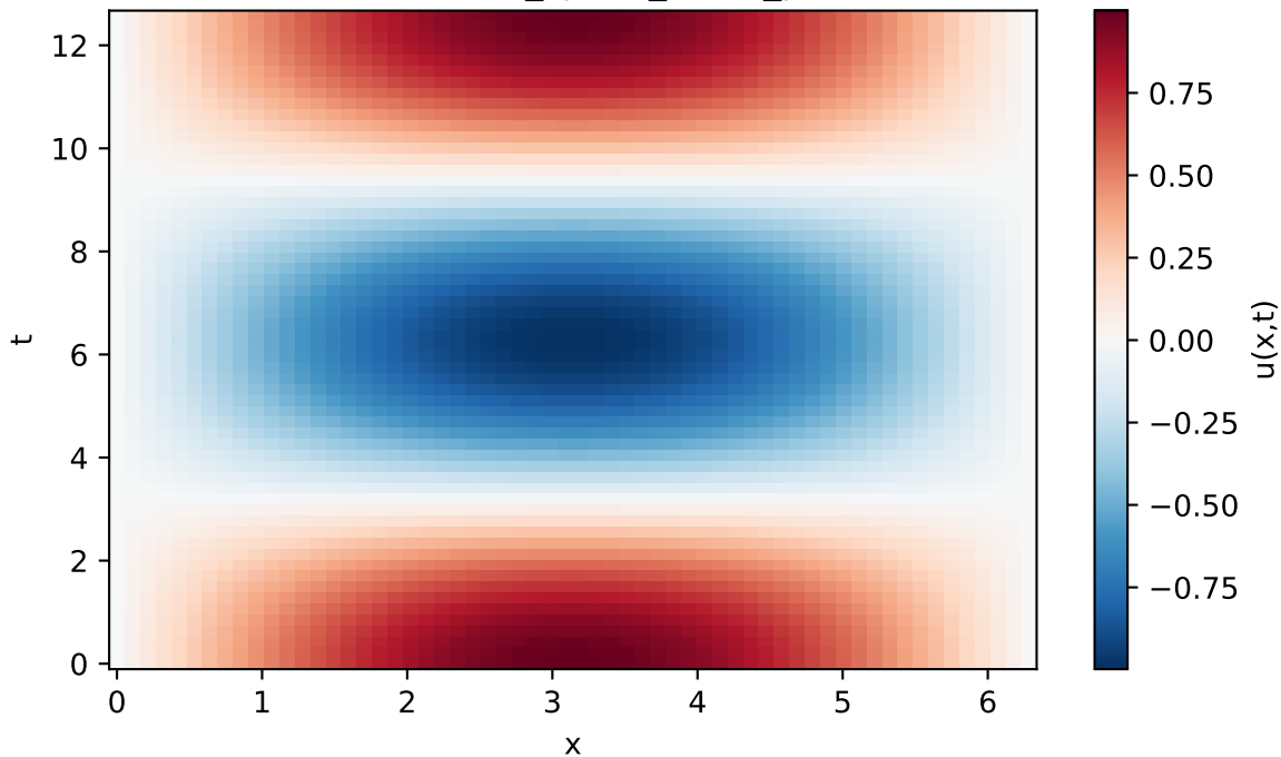
1D Wave - KANN_spline_same_params
