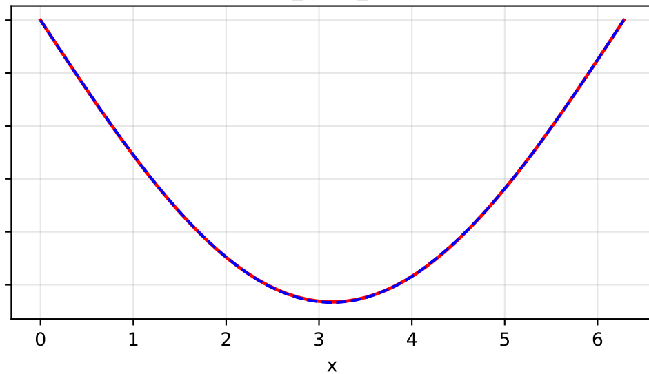
KANN_cheb_decay
