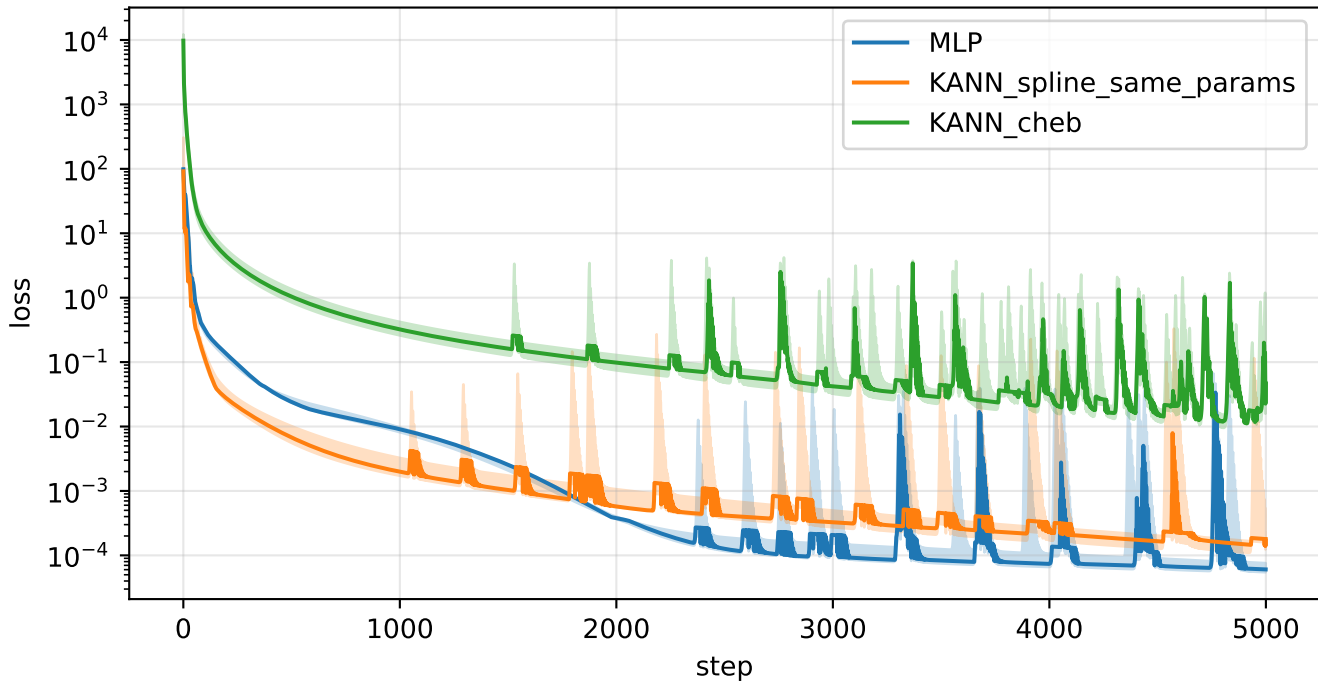
2D Poisson - loss (median over 3 seeds)
