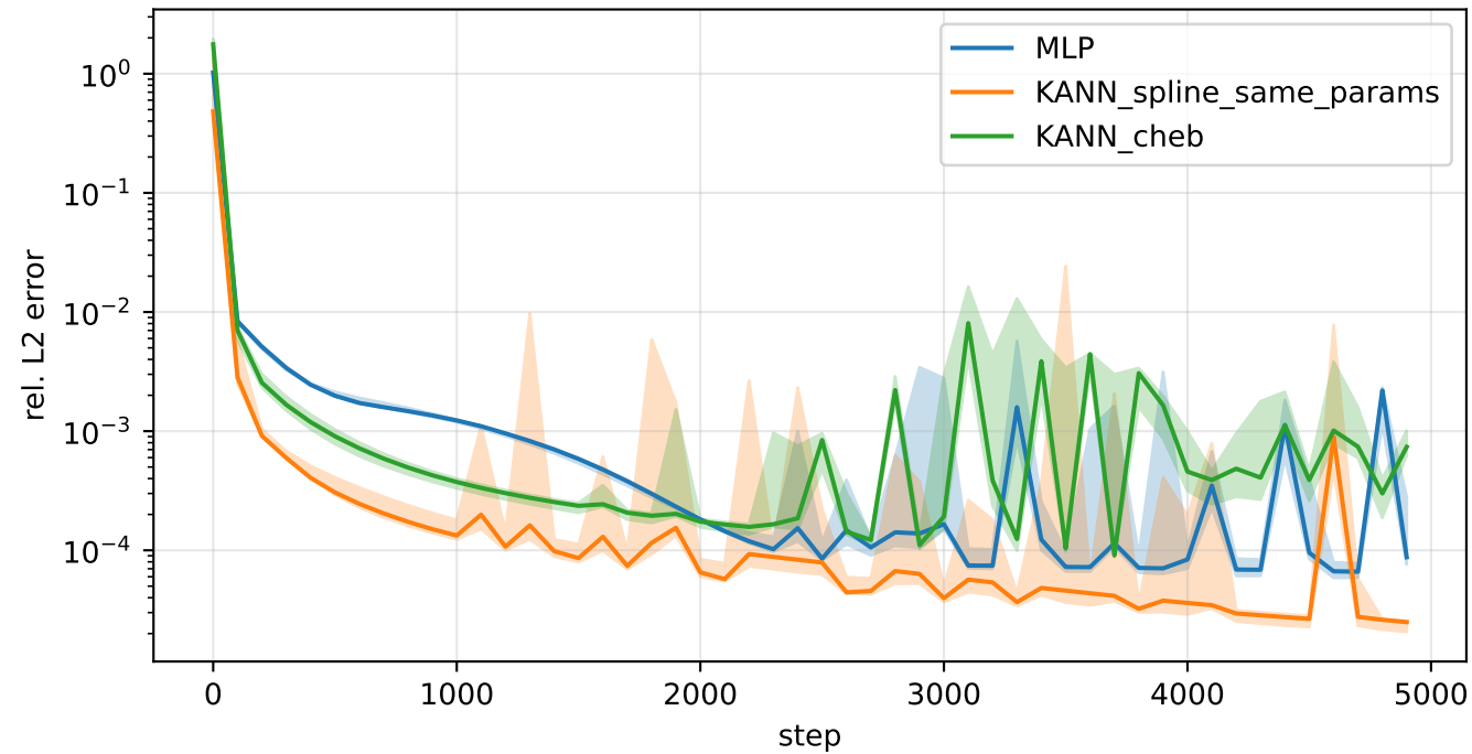
2D Poisson - relative L2 error (median over 3 seeds)
