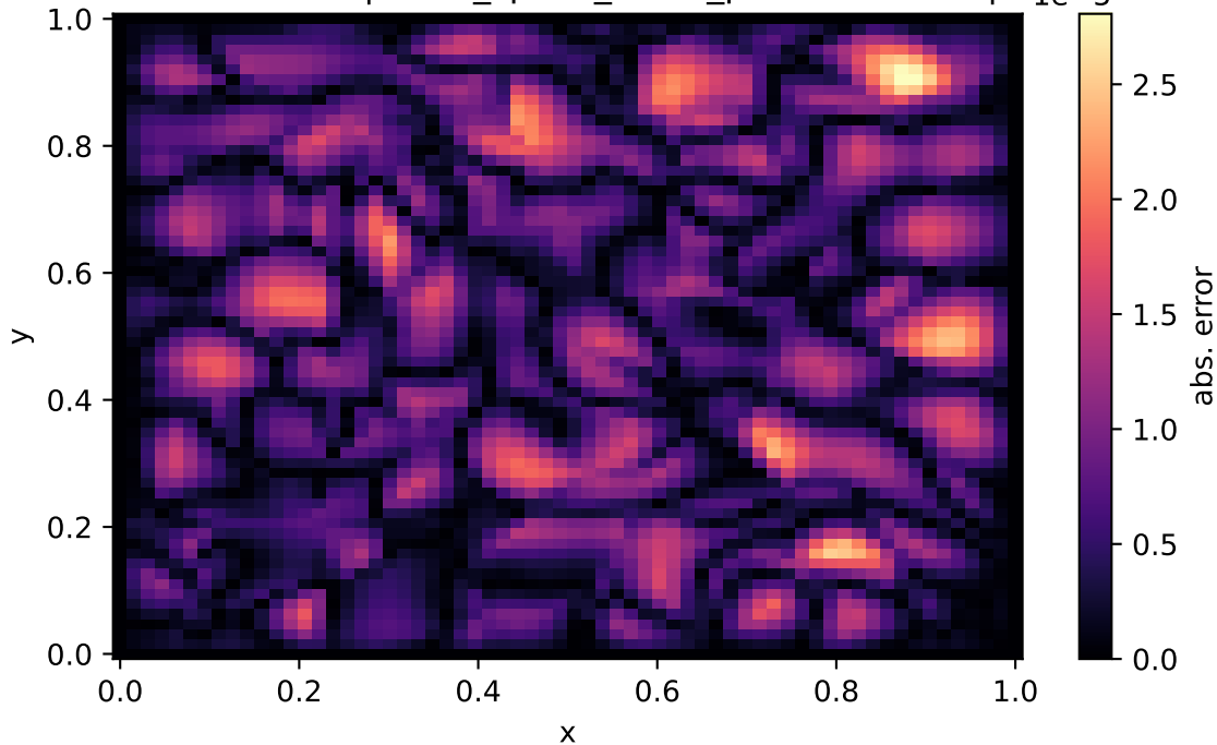
2D Poisson - |KANN_spline_same_params - exact|
