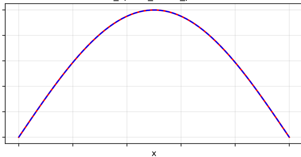
KANN_spline_same_params
