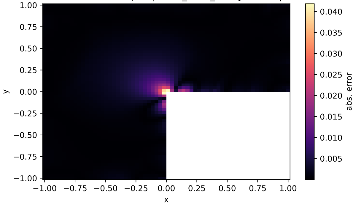
2D Poisson L-shape - |KANN_cheb_decay - exact|
