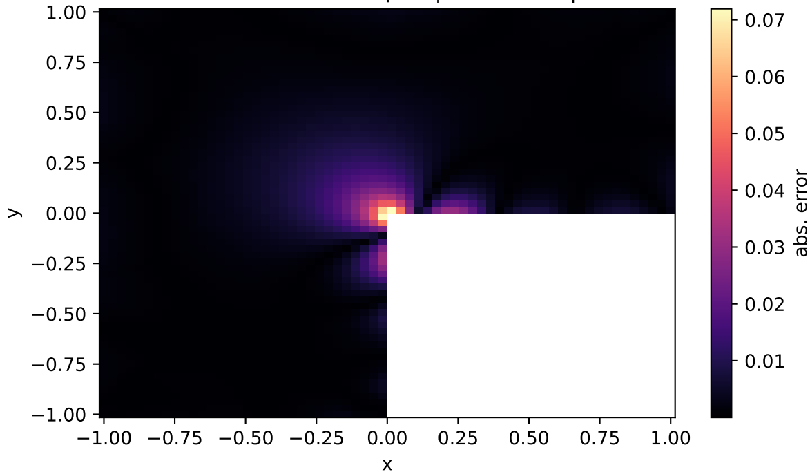
2D Poisson L-shape - |MLP - exact|
