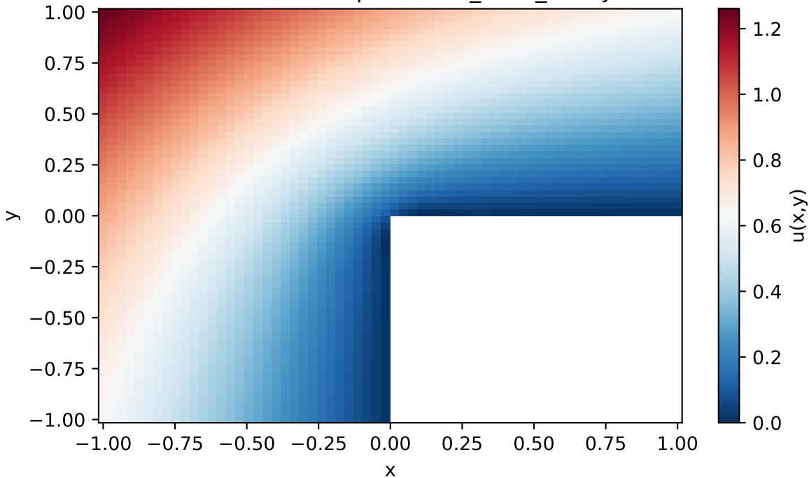
2D Poisson L-shape - KANN_cheb_decay
