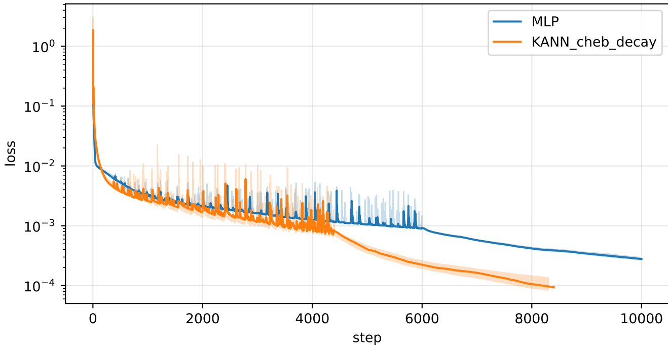
2D Poisson L-shape - loss (median over 3 seeds)
