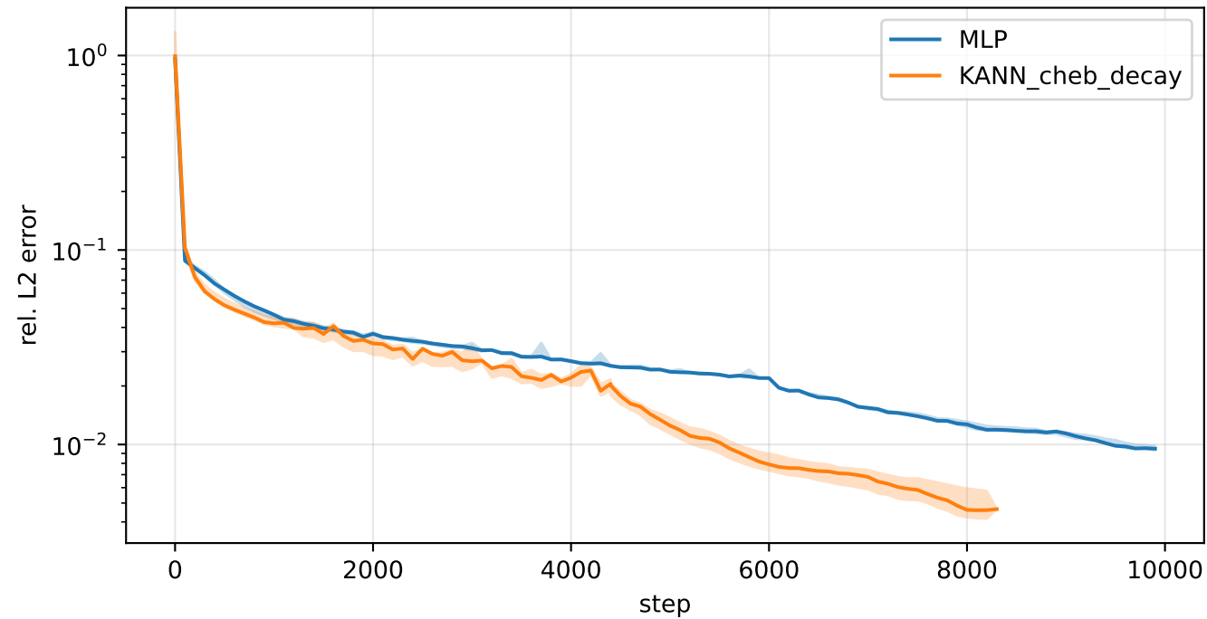
2D Poisson L-shape - relative L2 error (median over 3 seeds)
