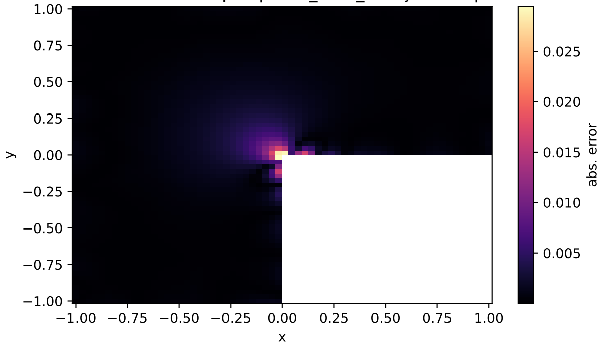
2D Poisson L-shape - |\text{KANN\_cheb\_decay} - \text{exact}|
