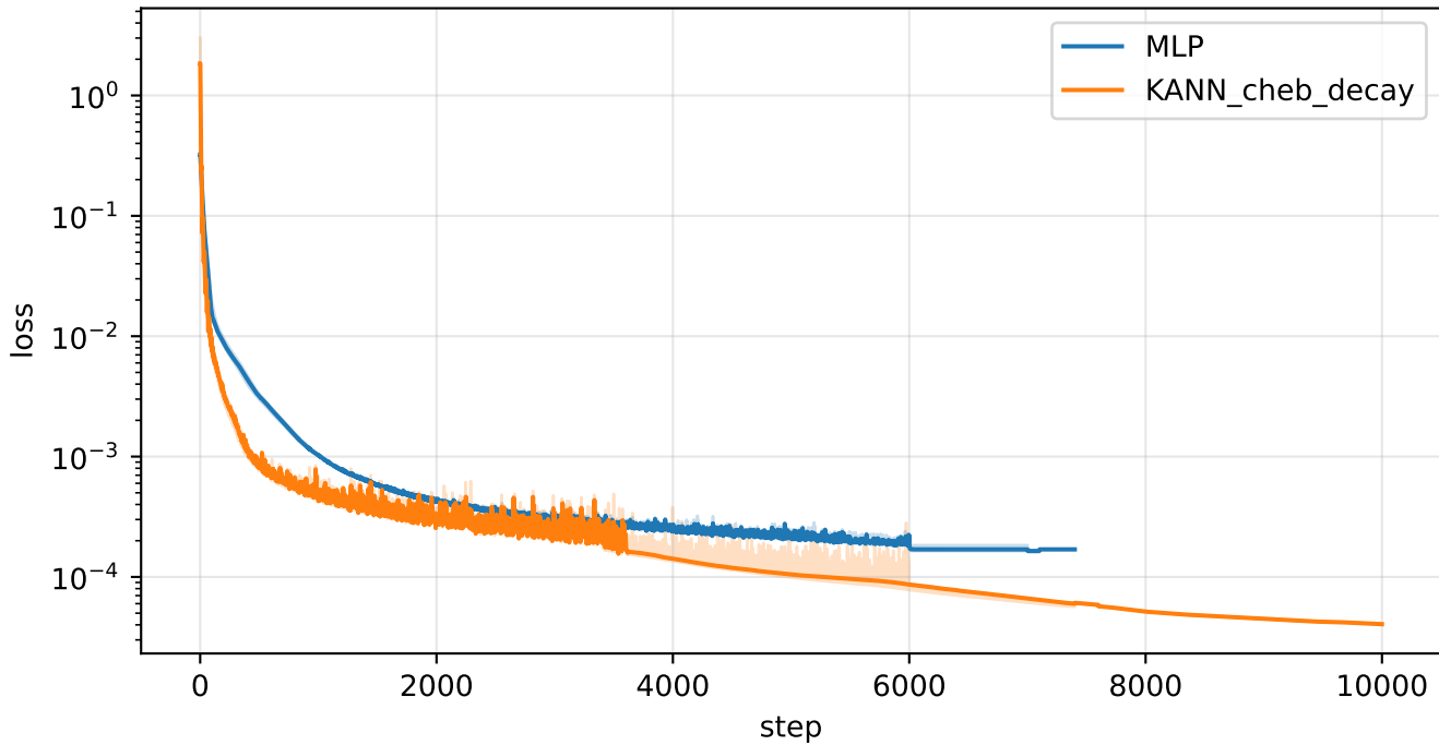
2D Poisson L-shape - loss (median over seeds)
