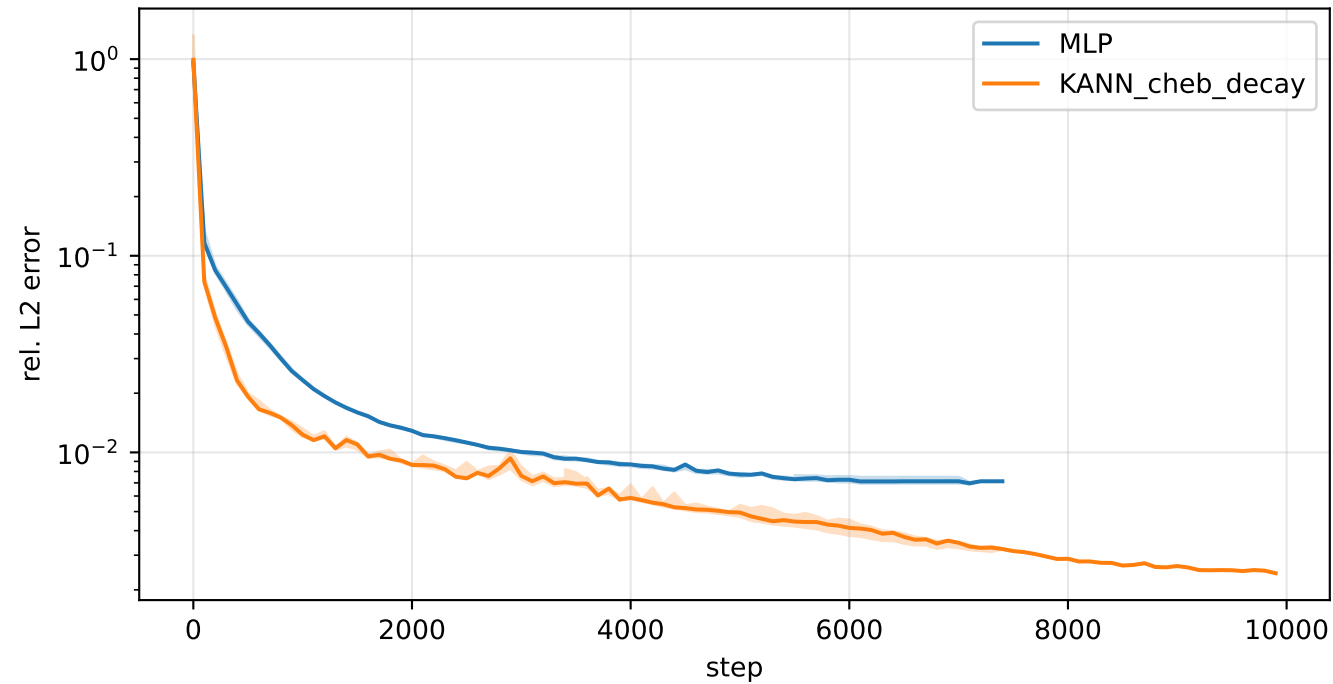
2D Poisson L-shape - relative L2 error (median over seeds)
