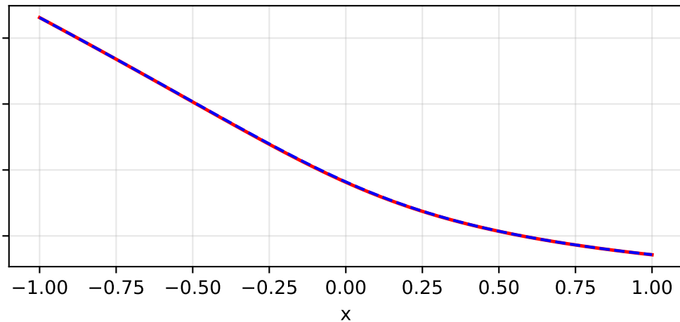
KANN_cheb_decay
