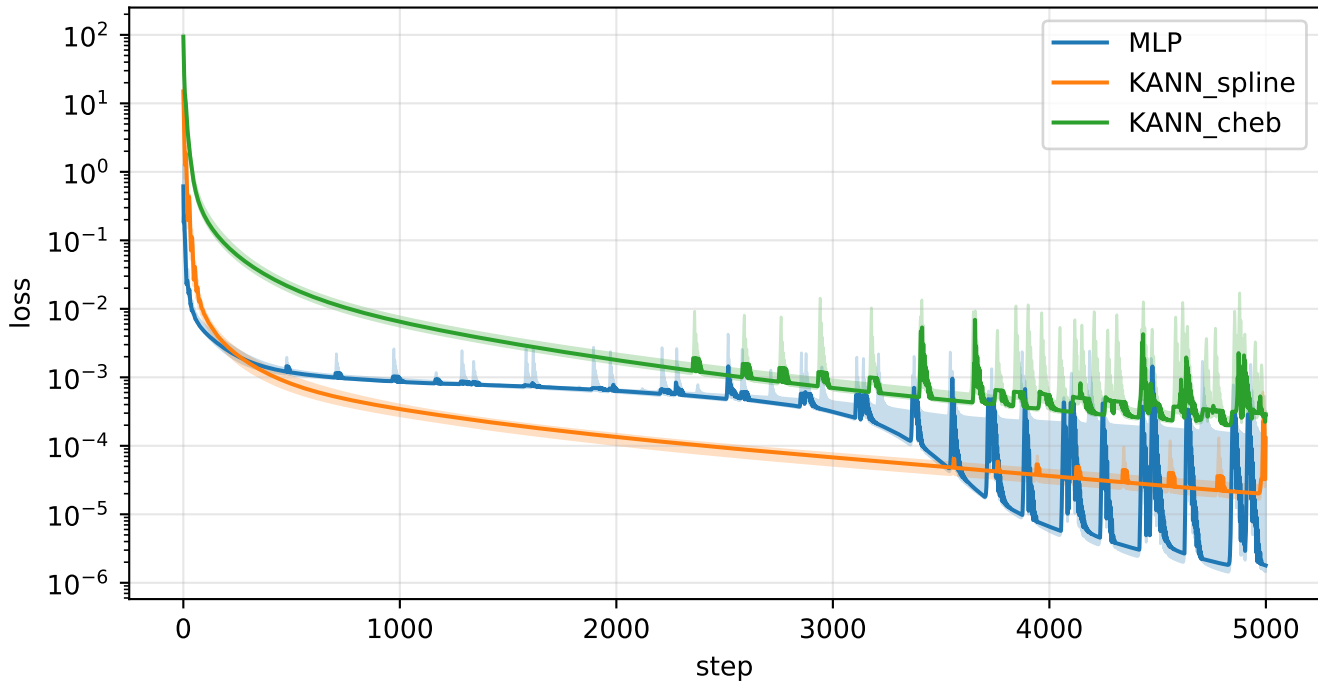
1D Wave Equation - loss (median over 3 seeds)
