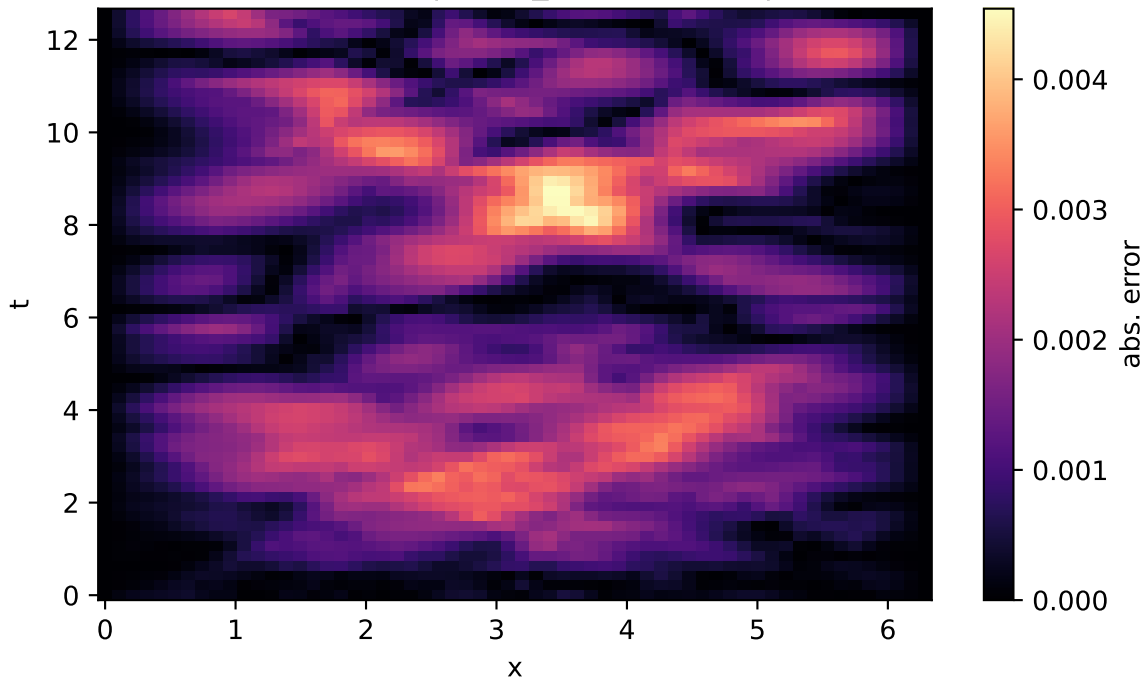
1D Wave - |KANN_spline - exact|
