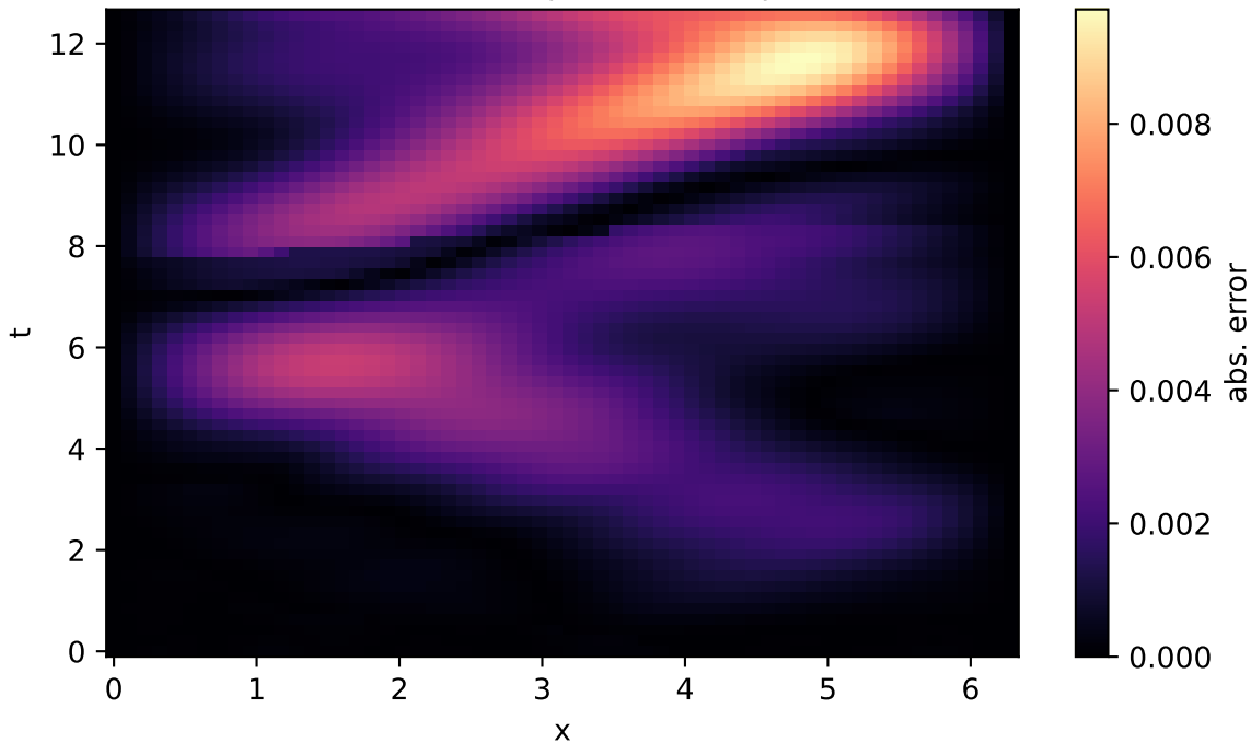
1D Wave - |MLP - exact|
