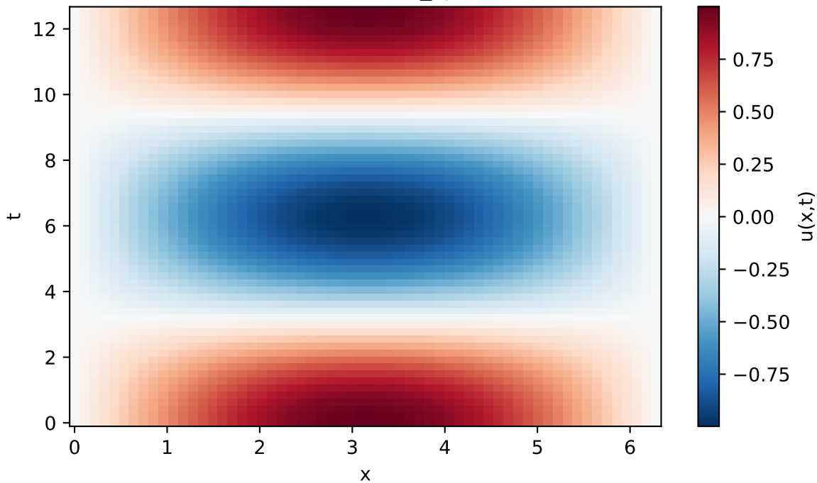
1D Wave - KANN_spline
