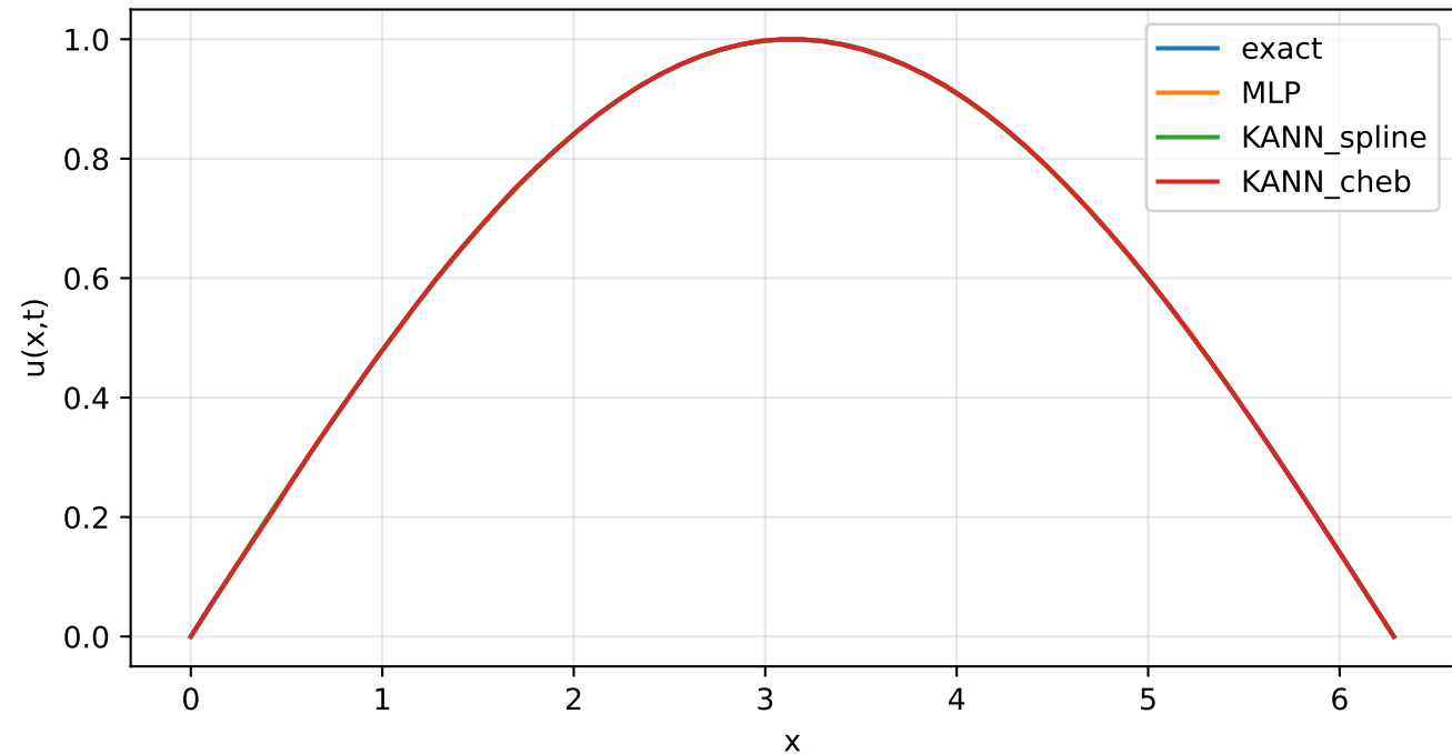
1D Wave at t = 0.00
