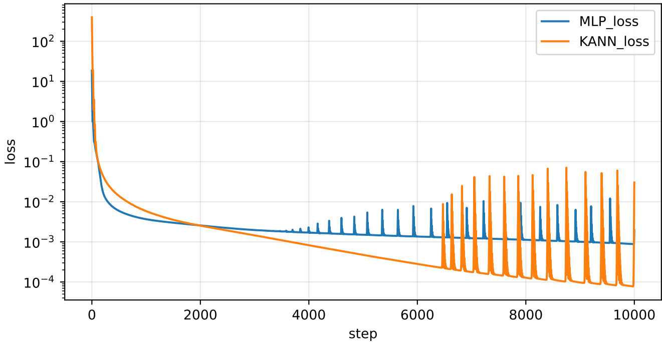
1D Wave Equation - MLP VS. KANN
