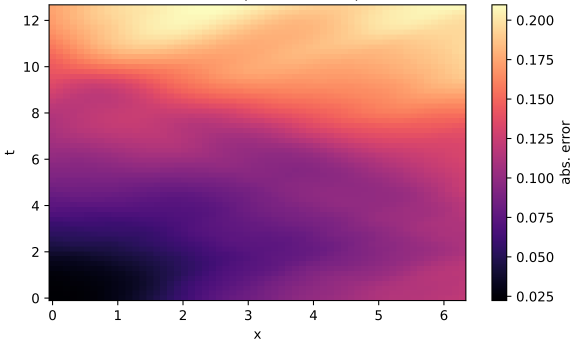
1D Wave - |KANN - exact|
