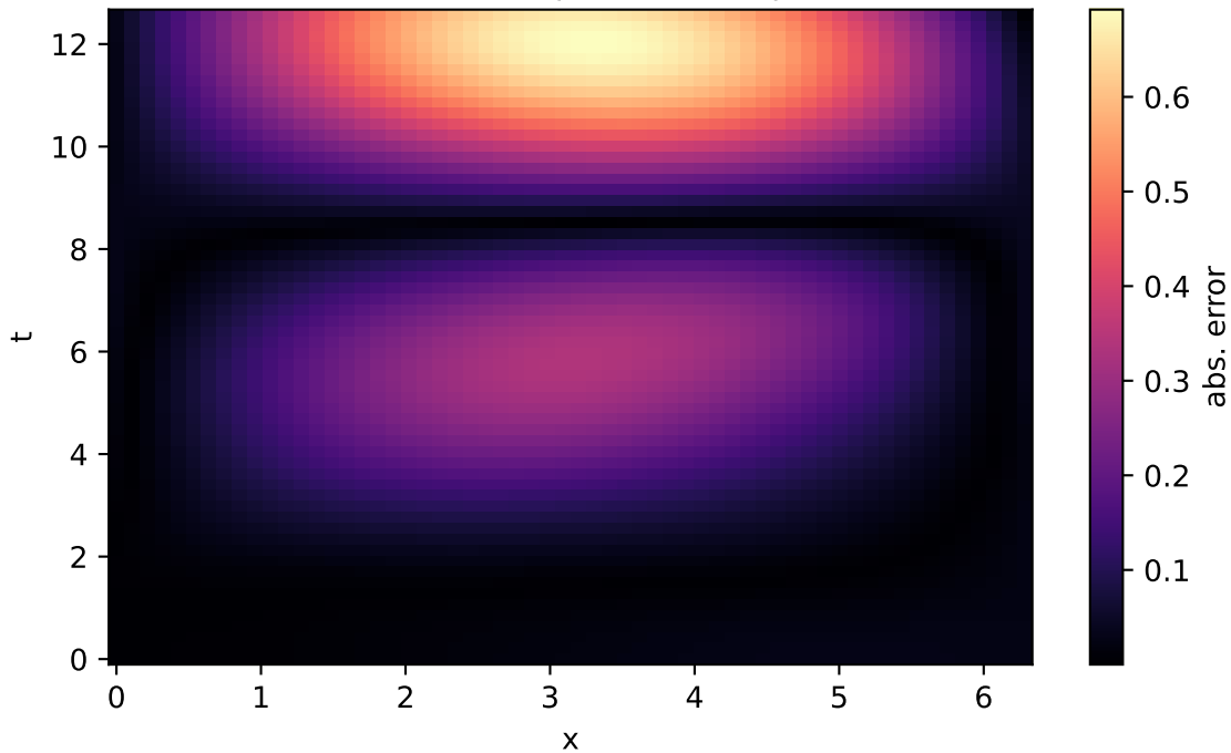
1D Wave - |\text{MLP} - \text{exact}|
