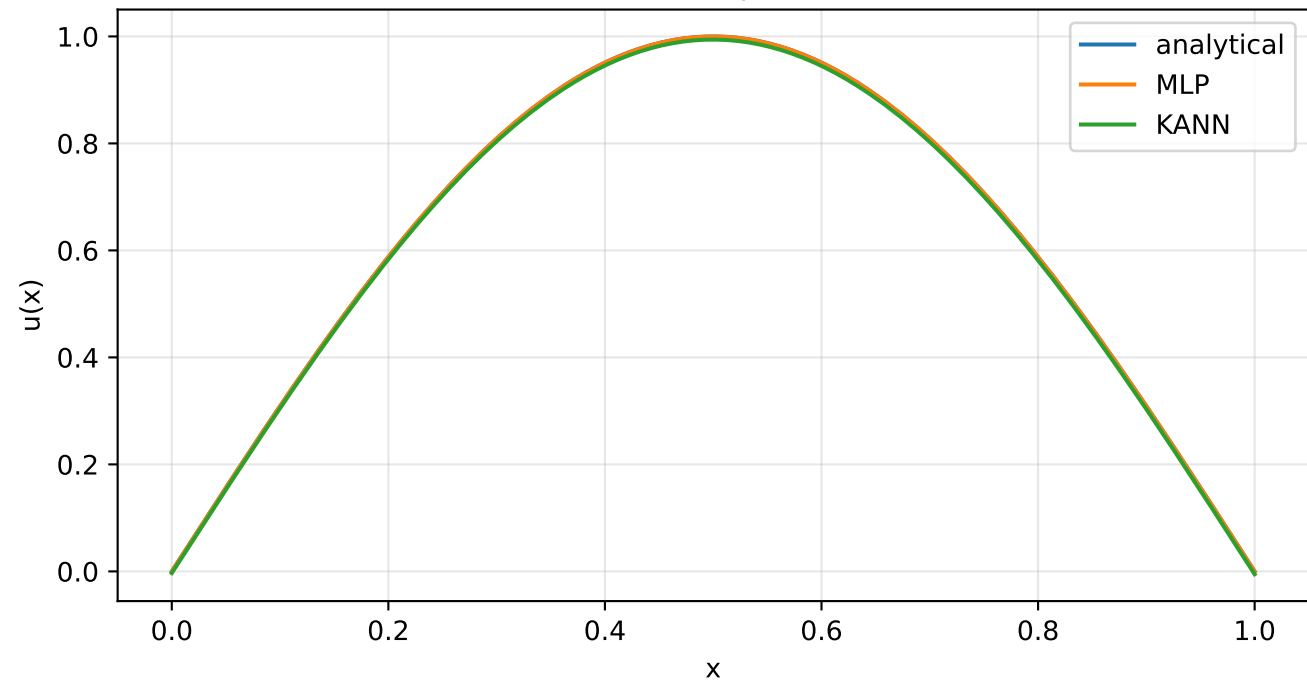
Poisson Equation
