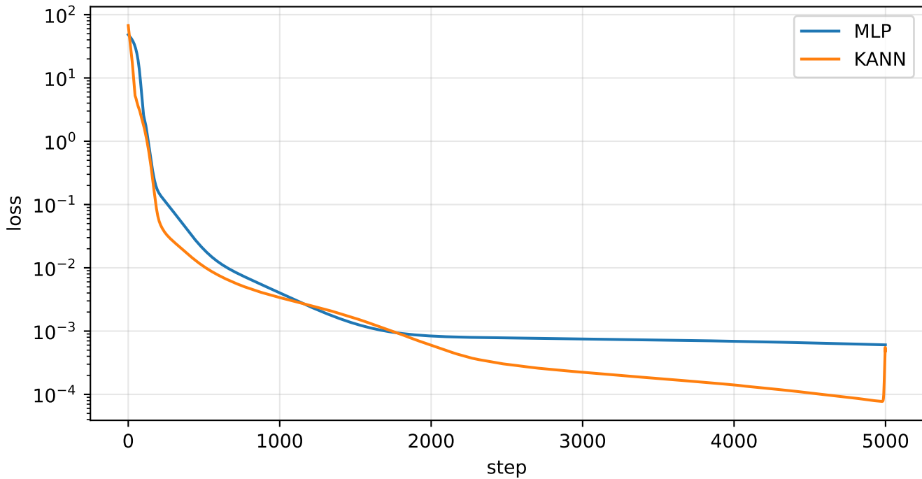
Loss 1D Poisson
